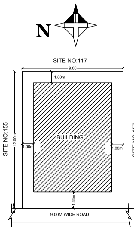
SITE PLAN
