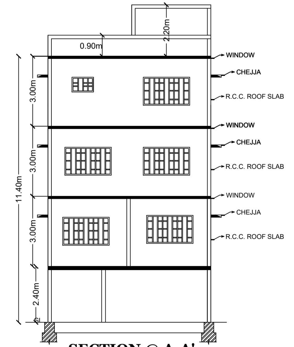
SECTION @ A-A'
